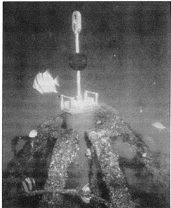
Figure 3. Self-recording gauge in mount
