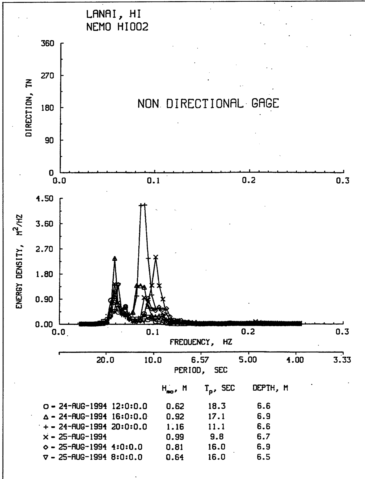
Figure D3. Wave spectra for Lanai, HI (H1002)
